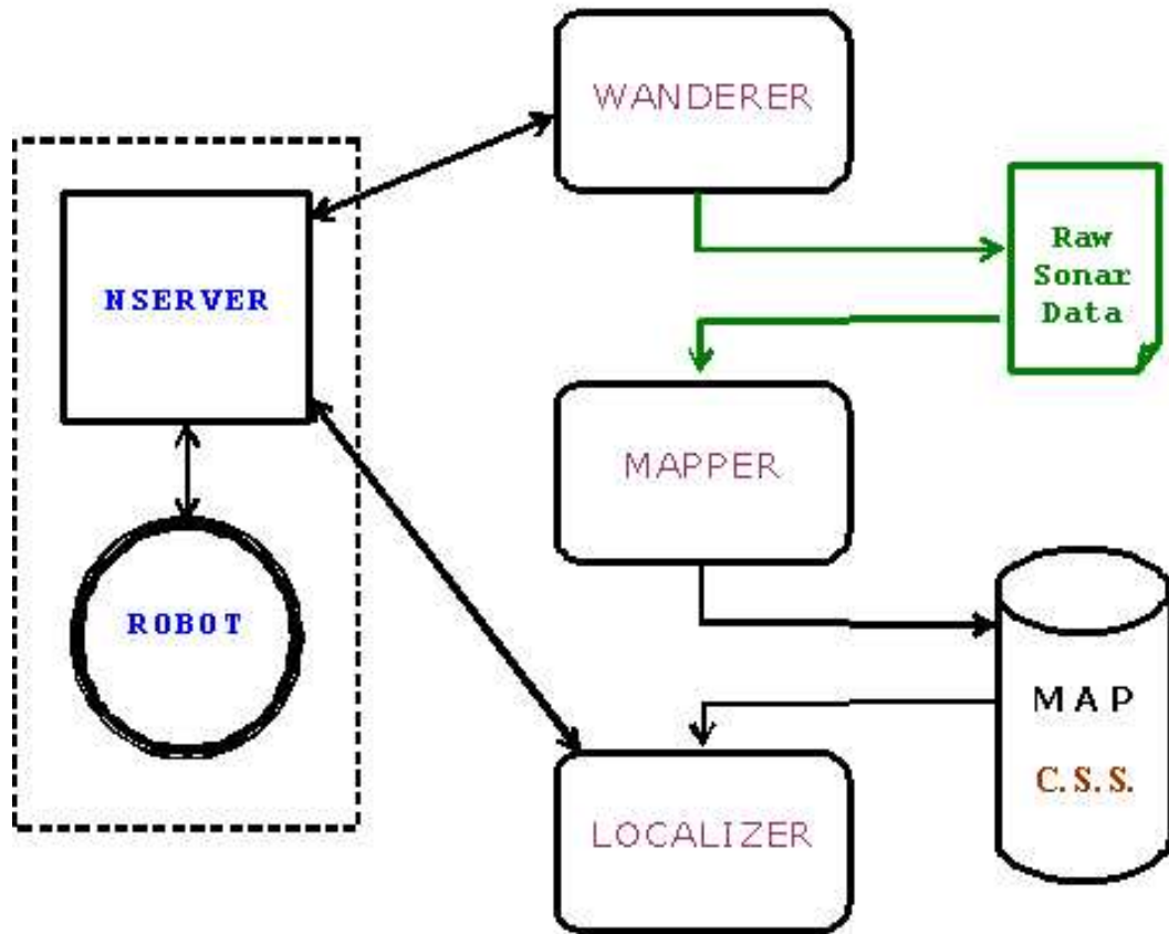
Figure 7.2: Component Diagram
